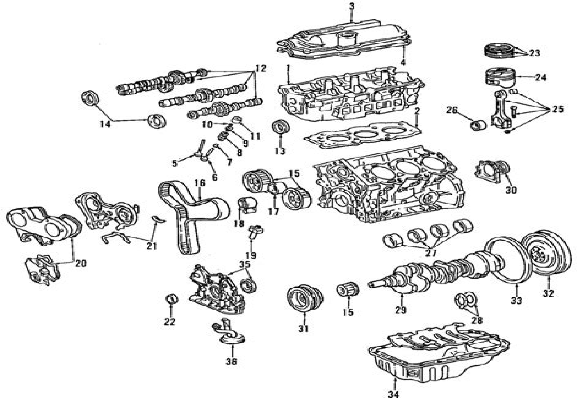
ENGINE - GAS, 6 CYLINDER, 3.0 LITER, 3.3 LITER
