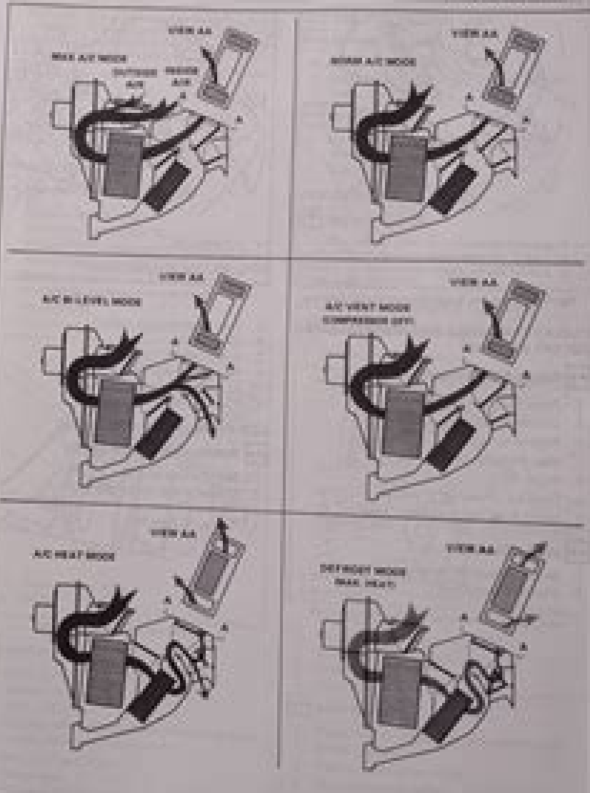
Figure 18-26 A/C Airflow Through Module in Each Mode
