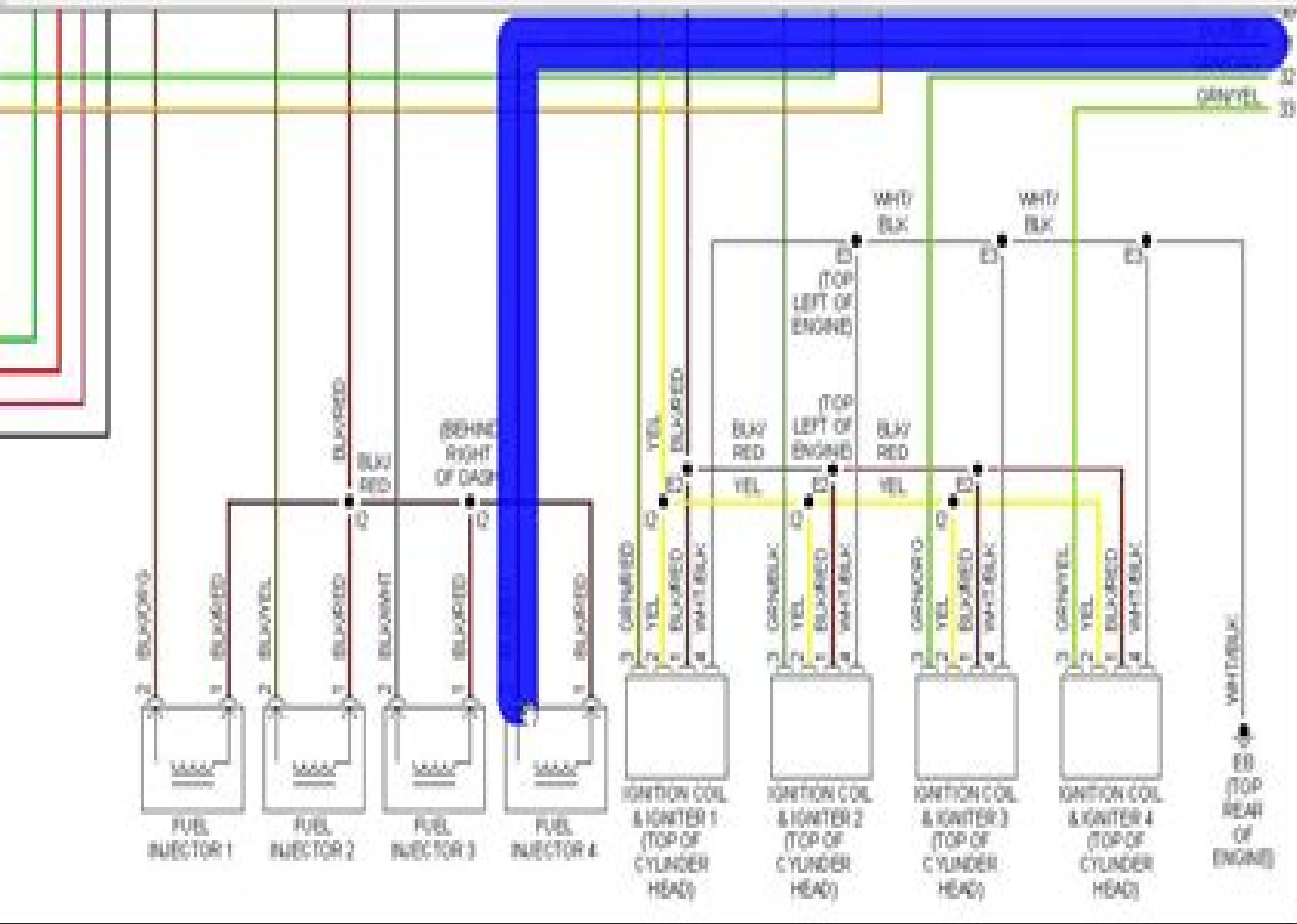
Fig. 10.1.10. Engine Performance Control (1 of 4)
