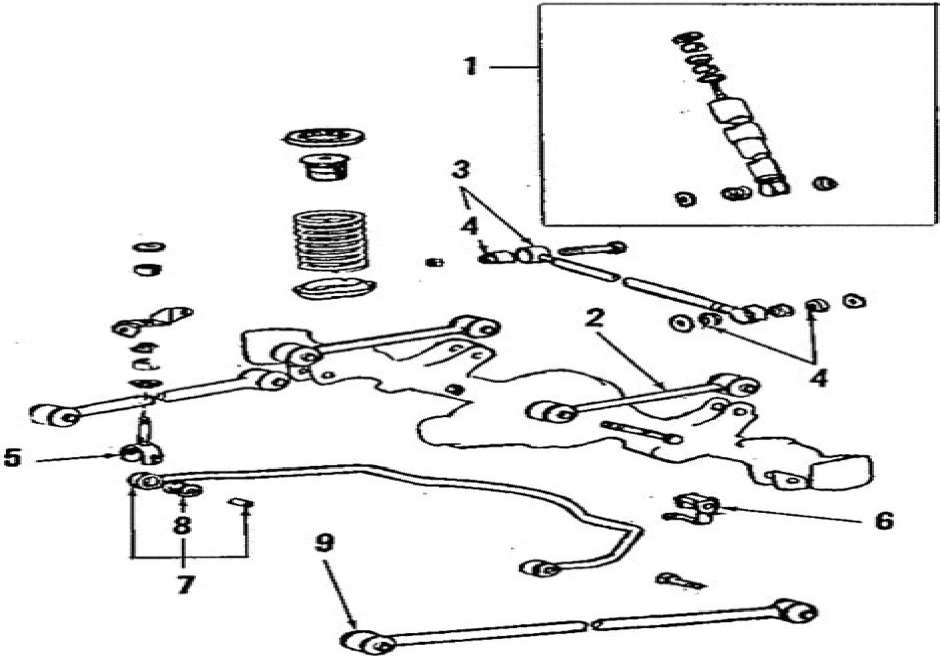
REAR SUSPENSION-4WD
