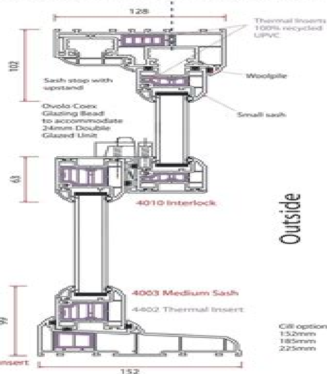
Vertical section through sash
