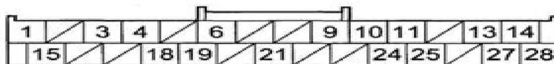
Fig. 34: Stereo Amplifier Connector B (28P) Connector End View Courtesy of AMERICAN HONDA MOTOR CO., INC.
