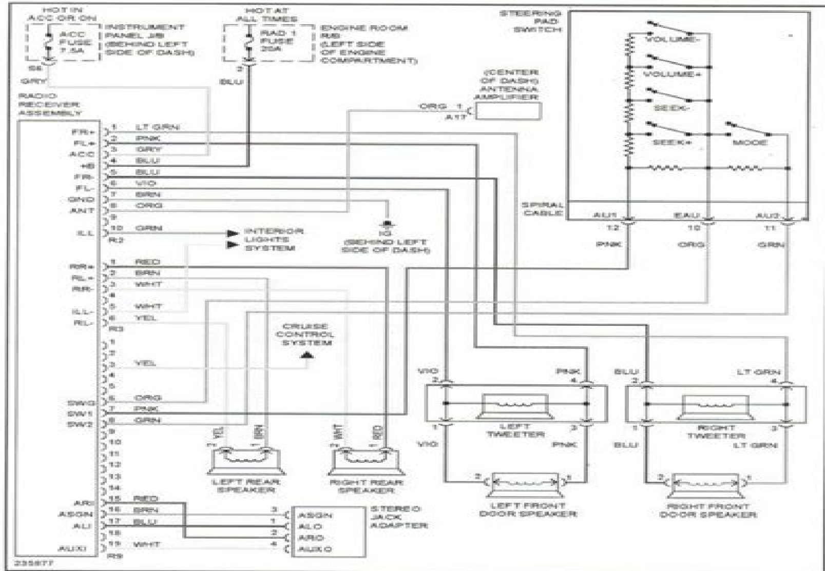
Fig. 32: Radio Circuit
