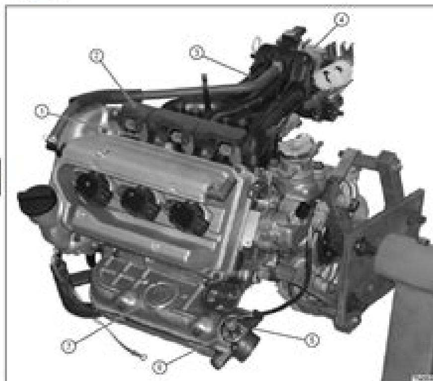
1 Injector (each) 2 Fuel Rail 3 Intake Manifold 4 Throttle Body Assembly 5 Exhaust Manifold 6 Oxygen Sensor 7 Heat Shield
