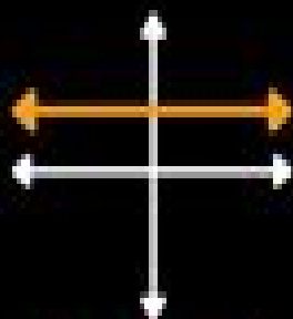
Constant
