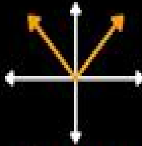
Absolute Value
