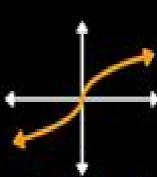
Cube Root
