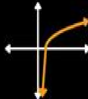
Logarithmic
