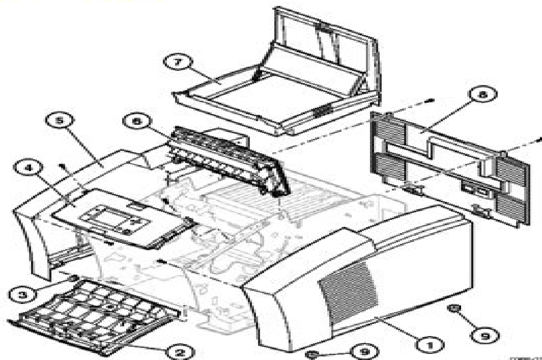
Fig 8-1 Cabinet FRUs
