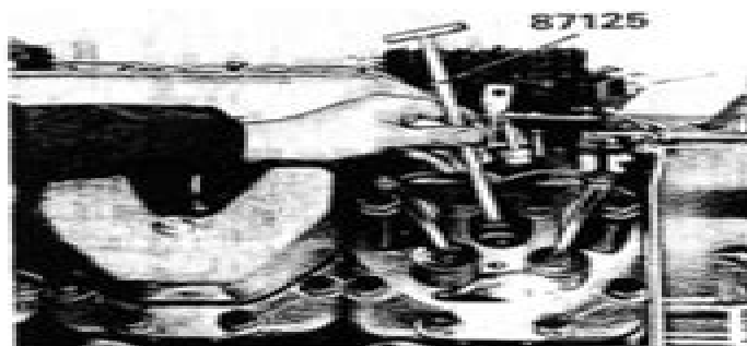
Removal of seal washer for injector
