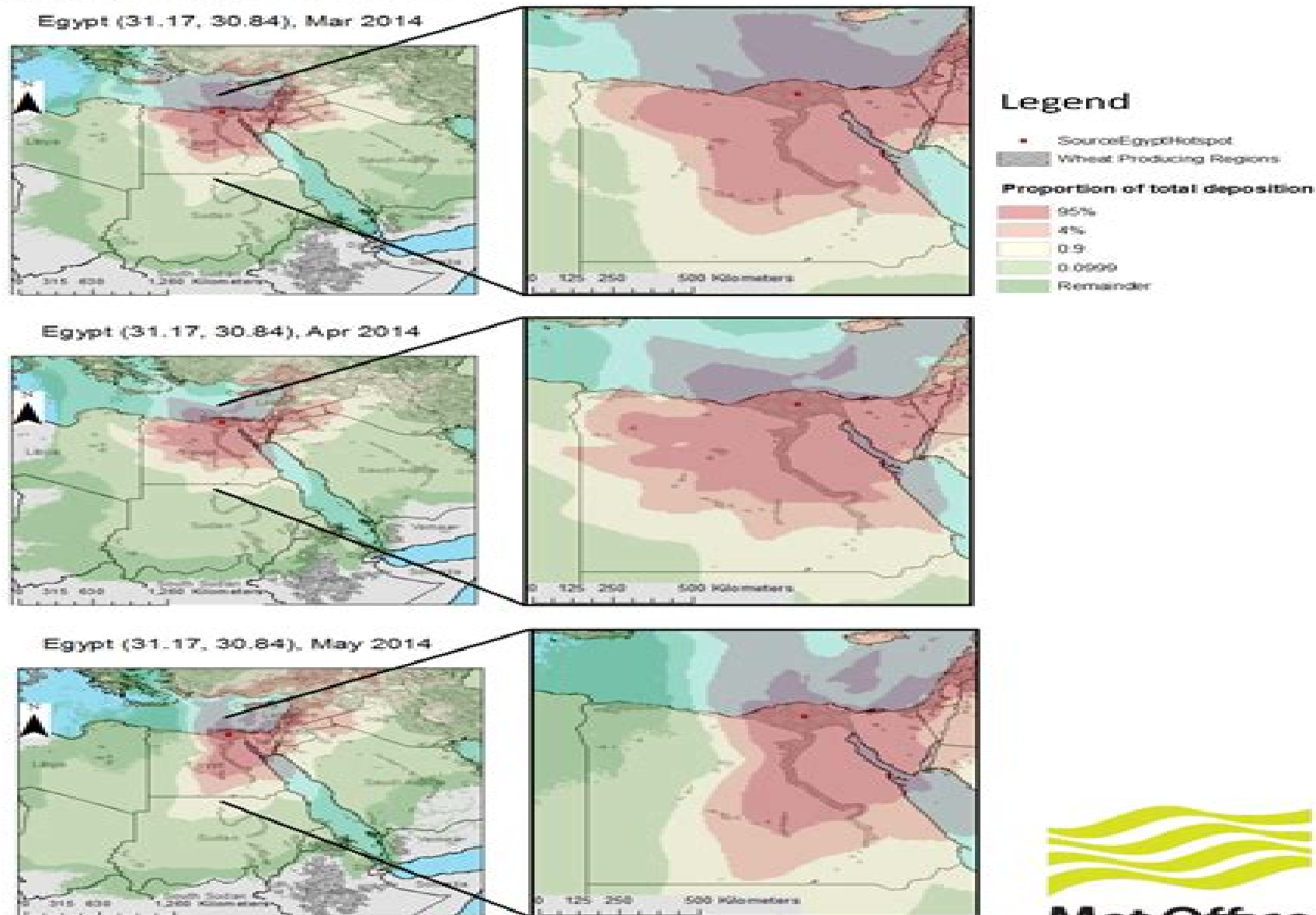
Fig 1: Modelled spore dispersal based on a source location in the central Nile Delta, Egypt for March, April, May 2014. Pink areas indicate where 95% of released spores are predicted to be deposited. Given high seasonal consistency, similar dispersal patterns would be expected to occur in March-May 2015.
