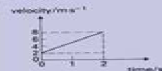
Figure 3.13 A velocity-time graph
