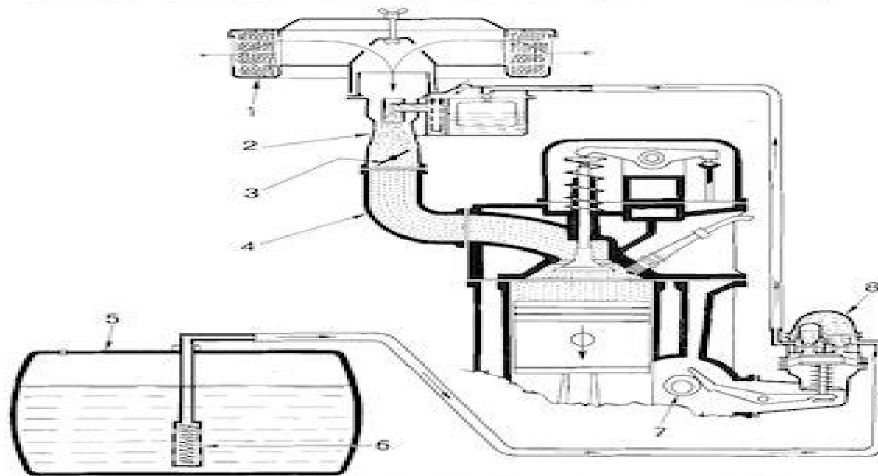
FIG. 1 Engine fuel and air feed systems: 1 Air cleaner - 2 Carburetor - 3 Throttle - 4 Intake manifold - 5 Fuel tank - 6 Fuel strainer - 7 Camshaft - 8 Mechanical lift pump.
