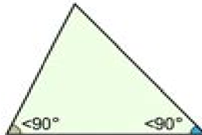
Acute
