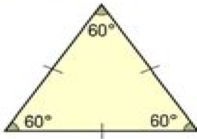
Equilateral
