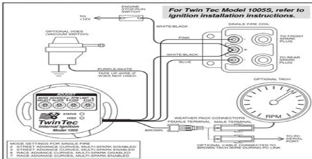
Figure 1 – Twin Tec Model 1005 Single Fire Wiring Diagram
