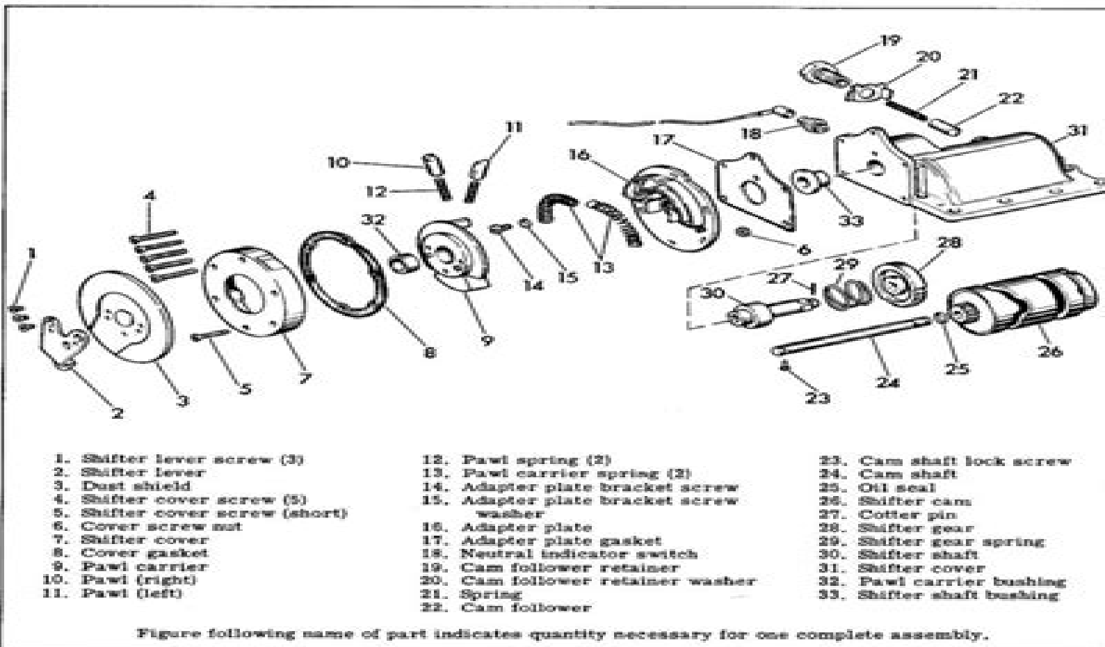
Figure 4D-6. Foot Shifter Cover - Exploded View
