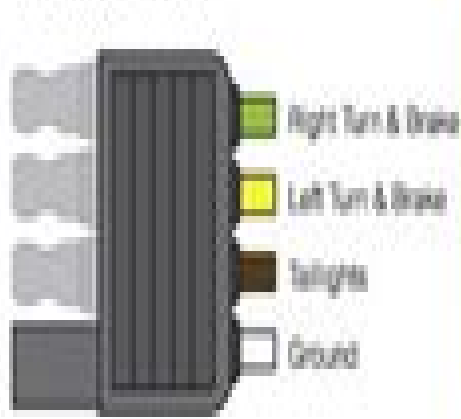
4 Wire Flat
