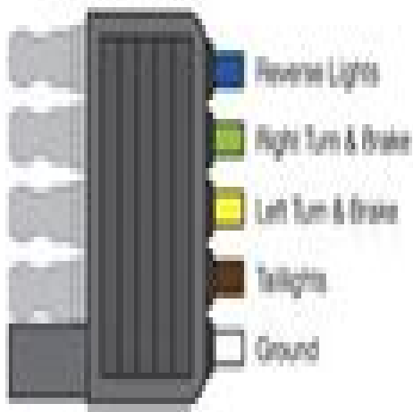
5 Wire Flat
