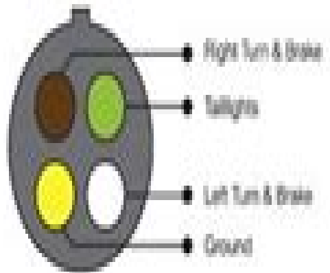
4 Pole Round
