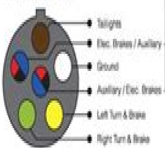
6 Pole Round
