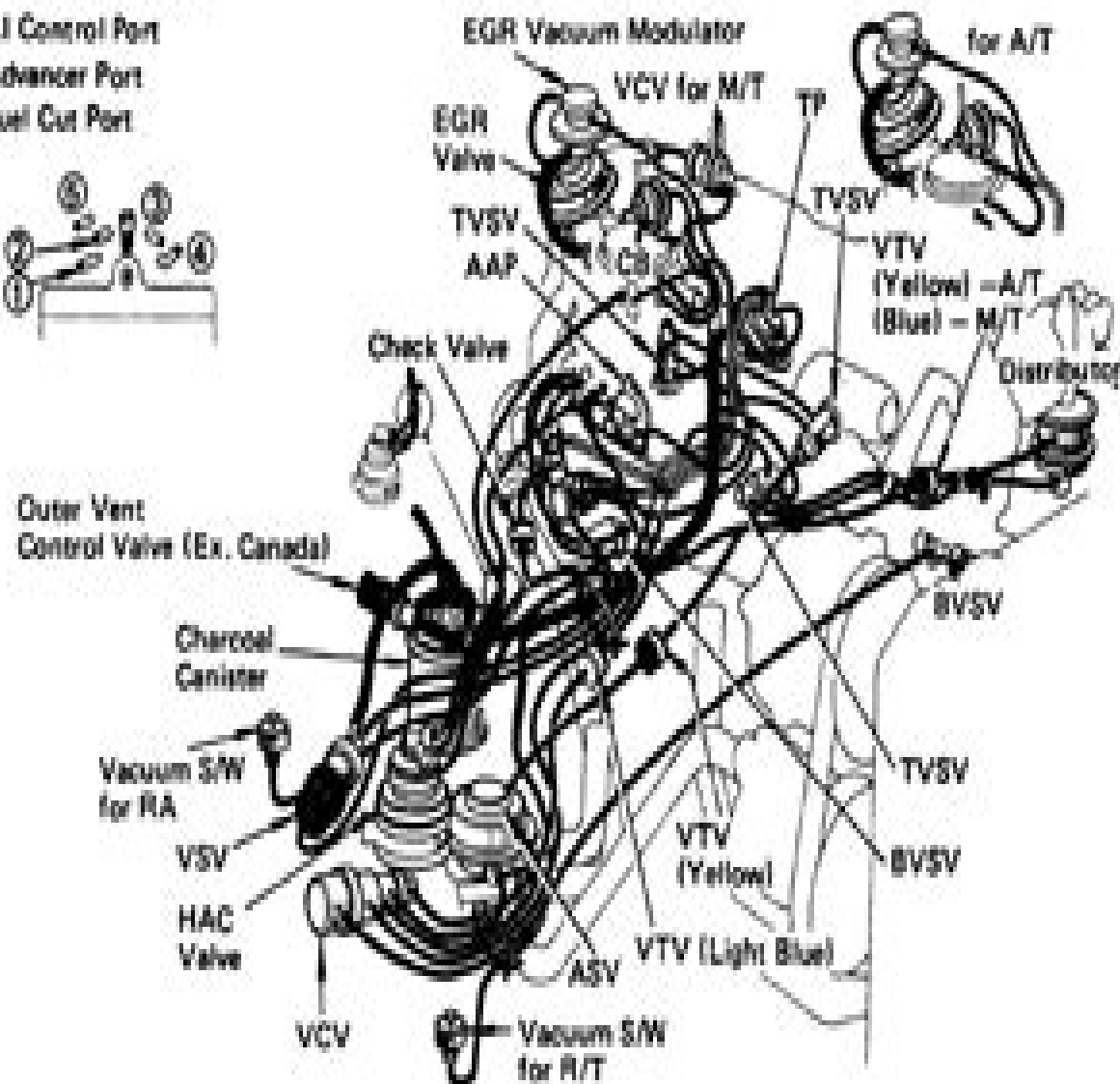
Fig. 60: 1978 Celica & Corolla (20R Engine) Exhaust Emission System (High Altitude)
