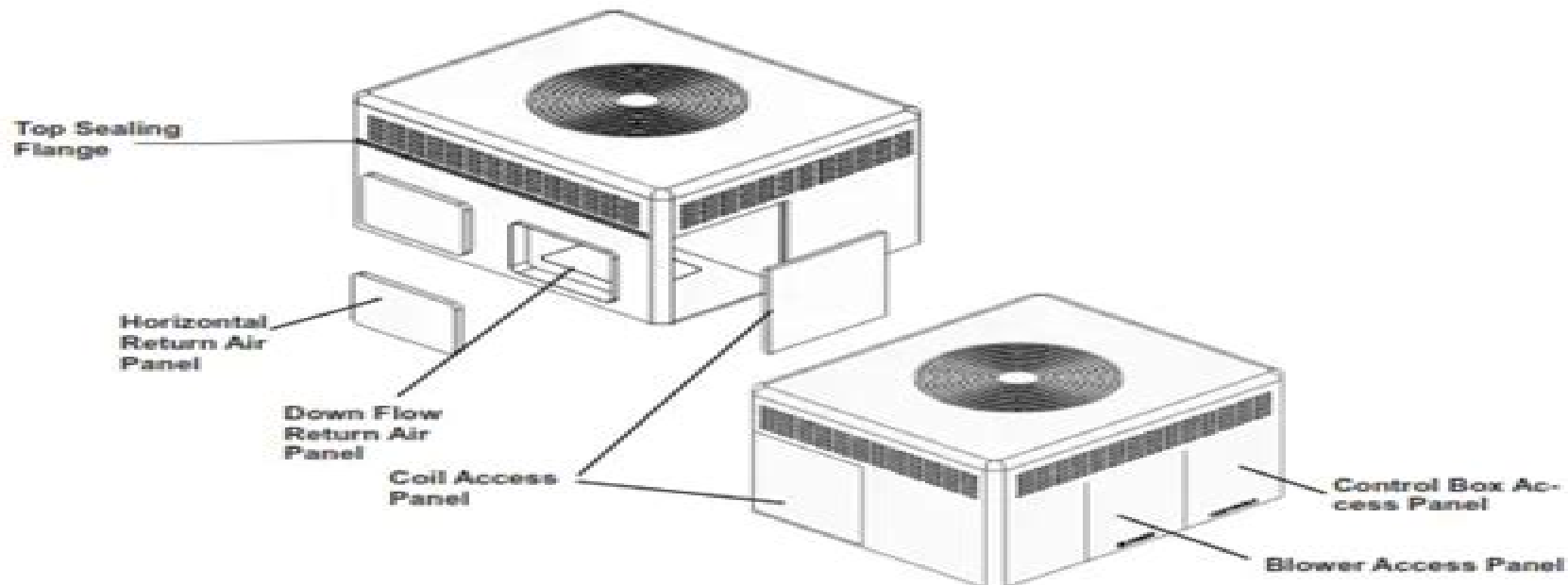
Figure 1. Remove Panels
