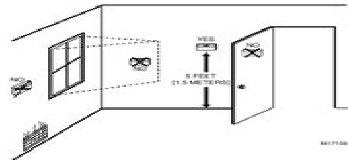
Fig. 1. Typical location of thermostat.
