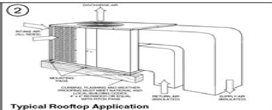
Typical Rooftop Application
