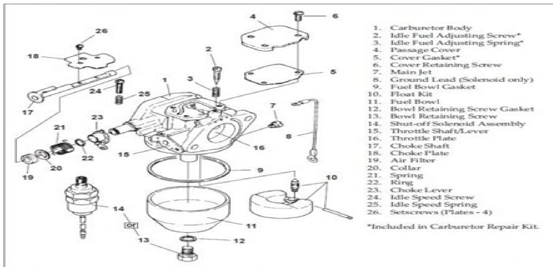
Figure 5-10. Typical Carburetor - Exploded View.
