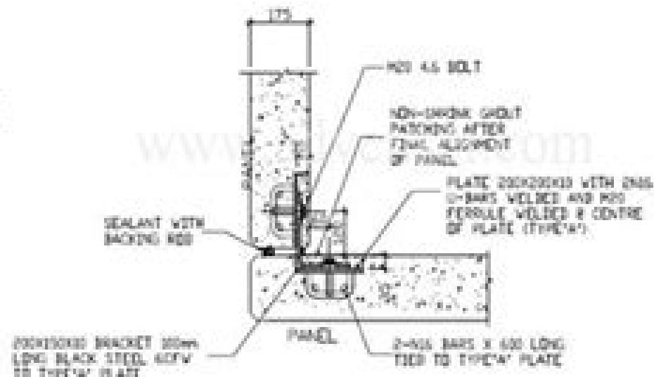
DETAIL 2 RECESSED PLATE CORNER CONNECTION (TYPE-B)
