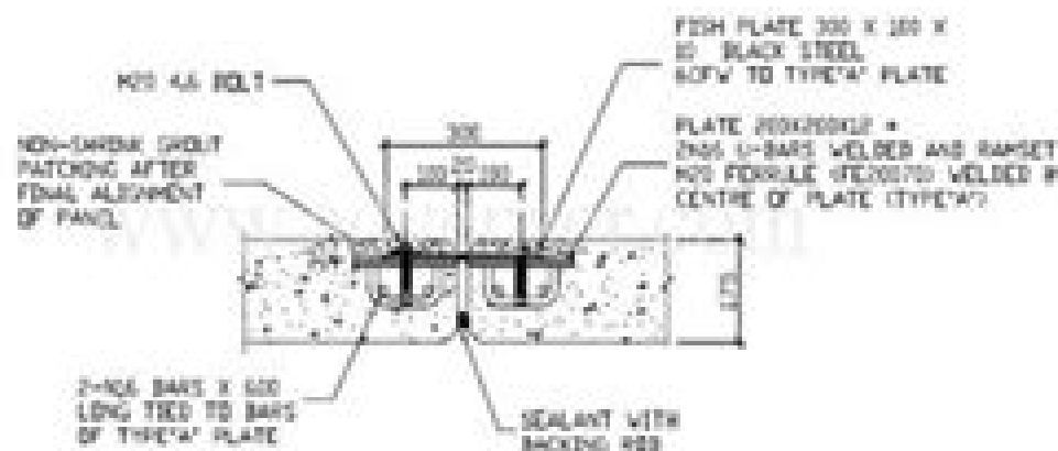
DETAIL 3 PANEL TO PANEL RECESSED PLATE CONNECTION DETAIL (TYPE-A)
