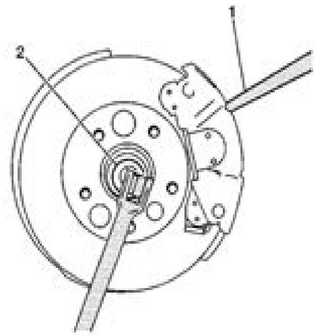
Fig. 3: Preventing Rotor Turning Using Drift Or Punch Courtesy of GENERAL MOTORS CORP.
