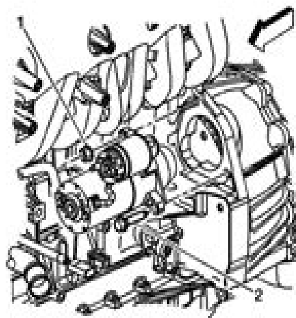
Fig. 31. Reversing/Installing Starter Motor Courtesy of GENERAL MOTORS CORP.
