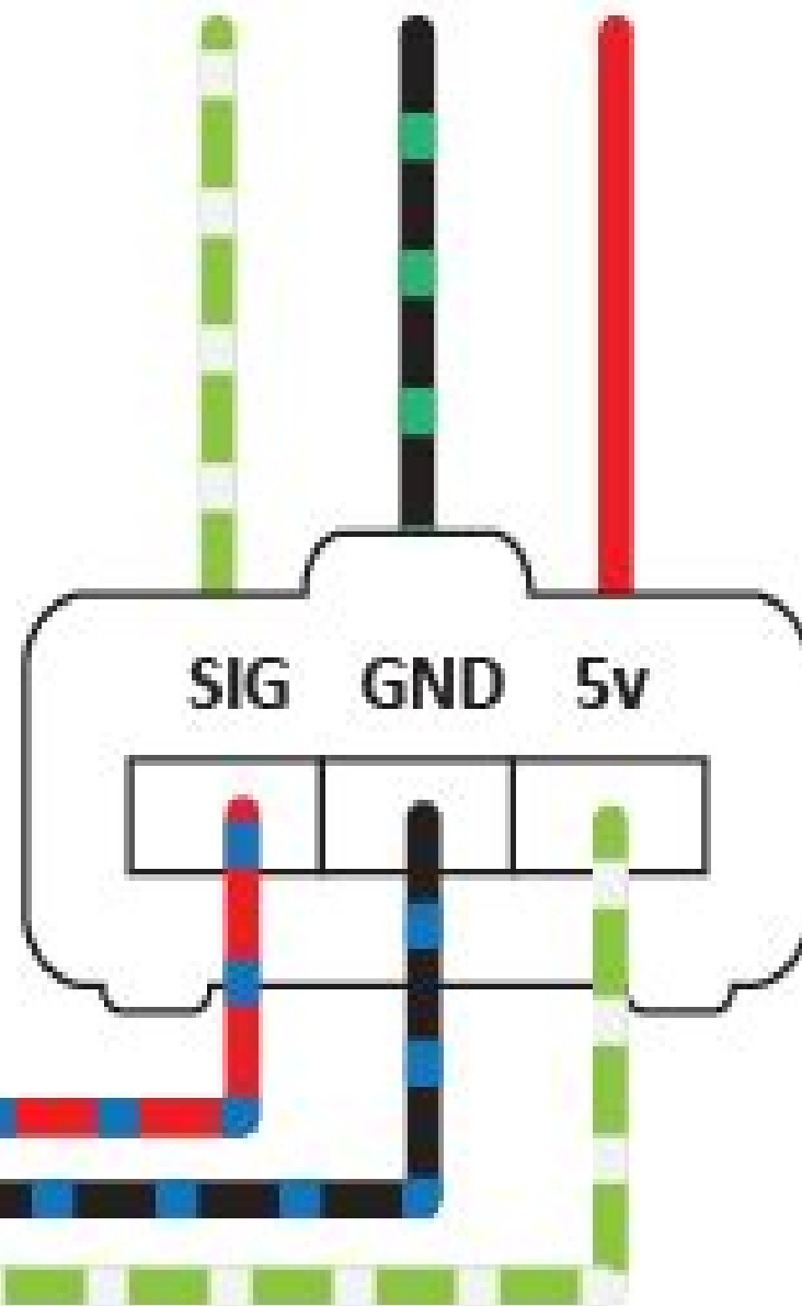
OE TPS Harness
