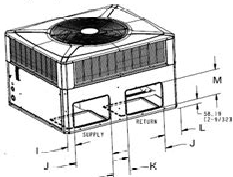
BACK DUCT OPENINGS
