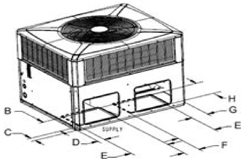
Figure 2. Bottom and Back Duct Openings
