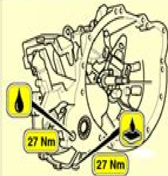
Manual gearbox
