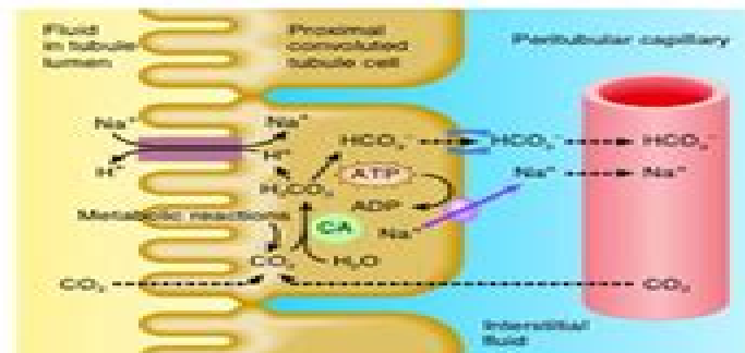
(a) \text{Na}^+ reabsorption and \text{H}^+ secretion
