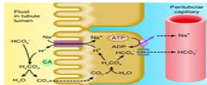
(b) \text{HCO}_3^- reabsorption
