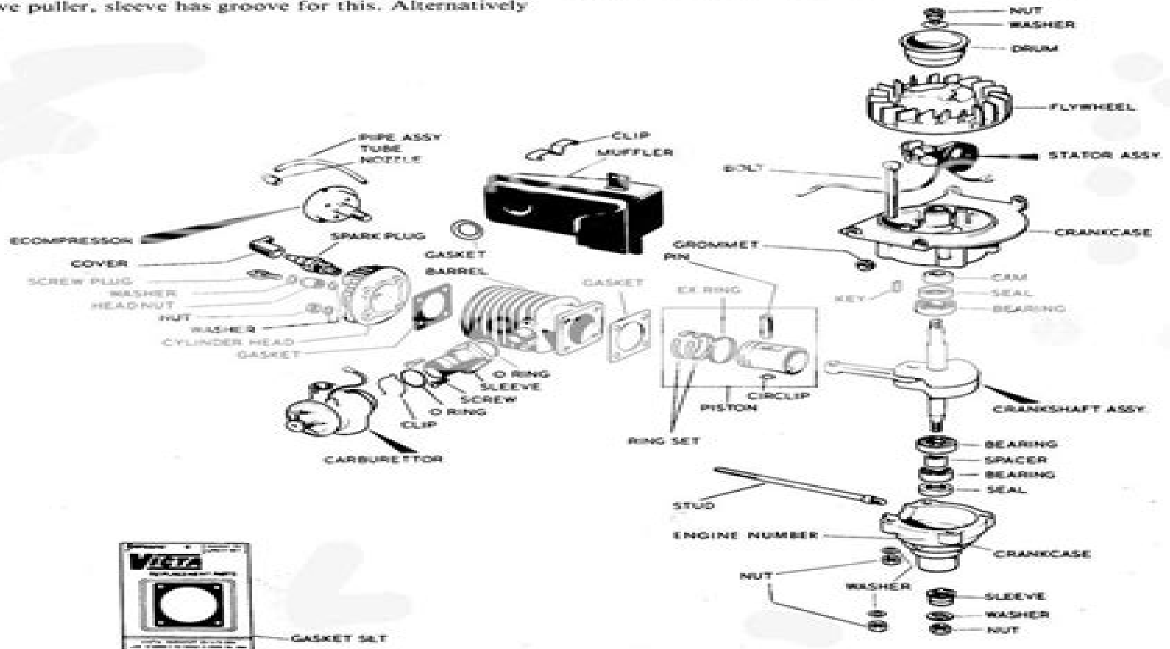
Dismantled view of late model 160cc engine fitted with breaker point ignition. Typical.
