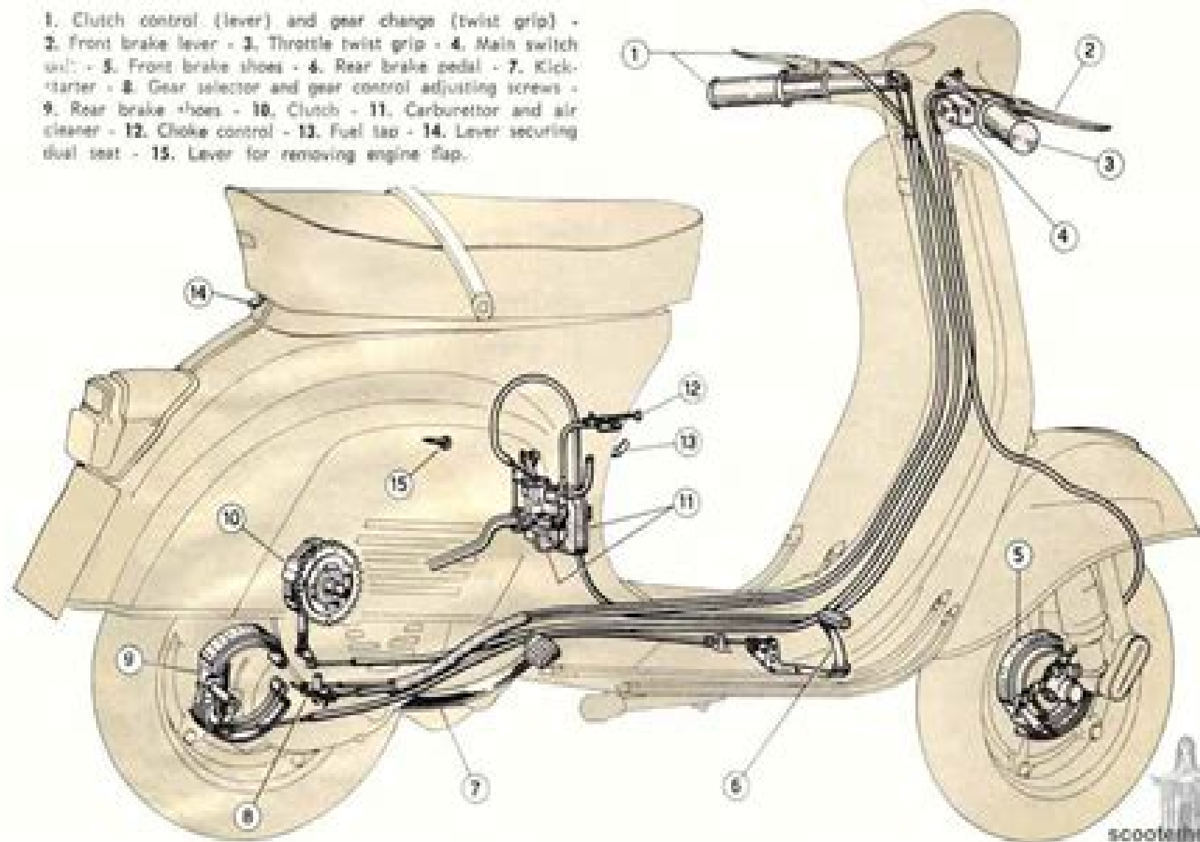
Fig. 2 - Installation of controls and transmission.
