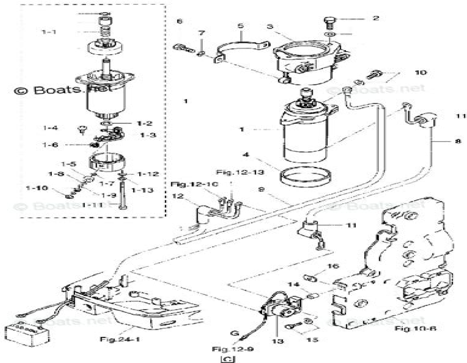
Fig. 11 ELECTRIC PARTS (STARTER MOTOR)
