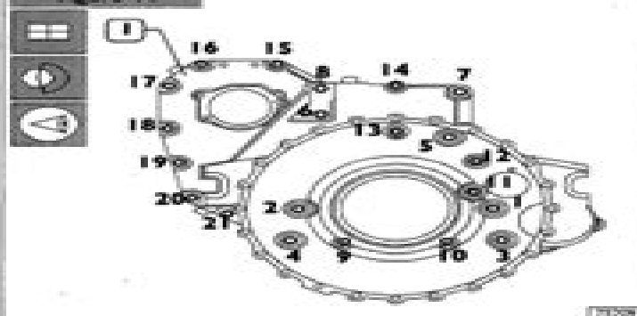
DIAGRAM SHOWING SCREW TIGHTENING TO FIX FLYWHEEL COVER BOX.
