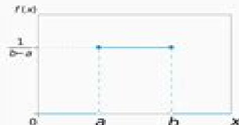
Uniform Distribution
