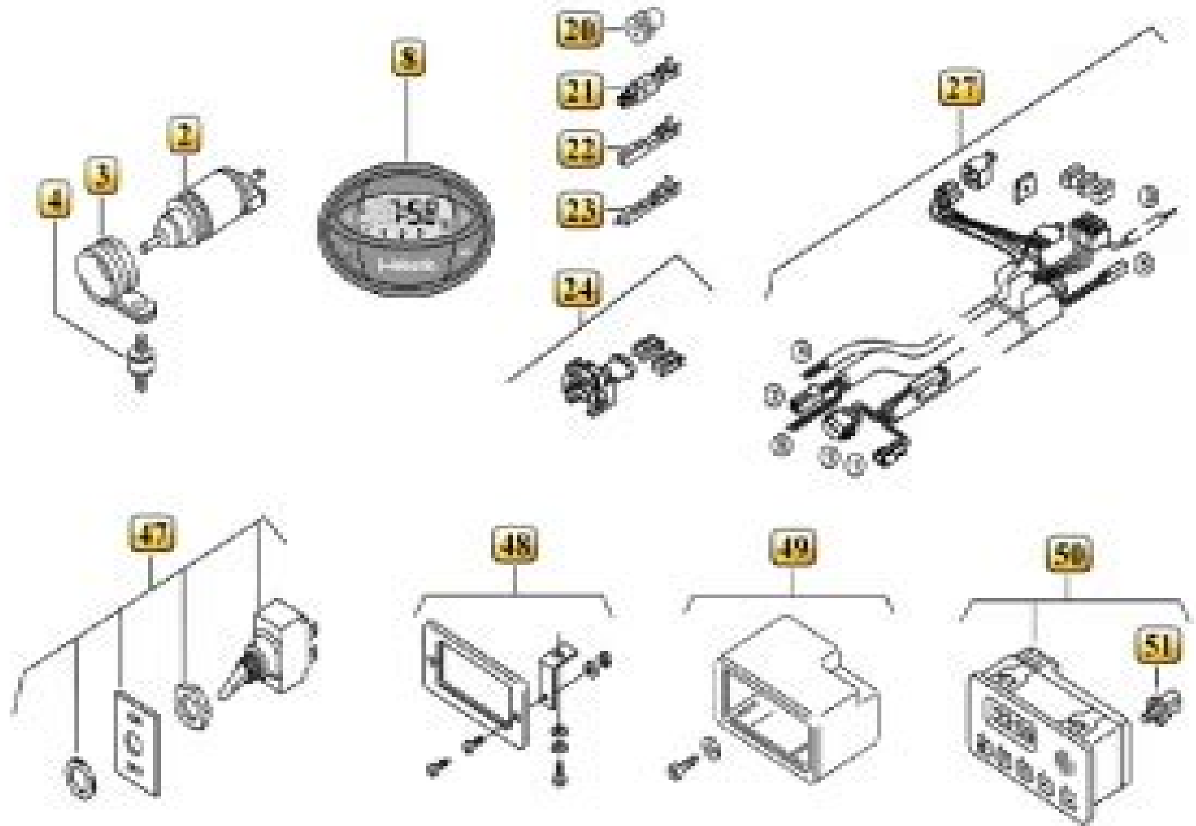
Thermo Top Z/C - B/D - fig. 2
