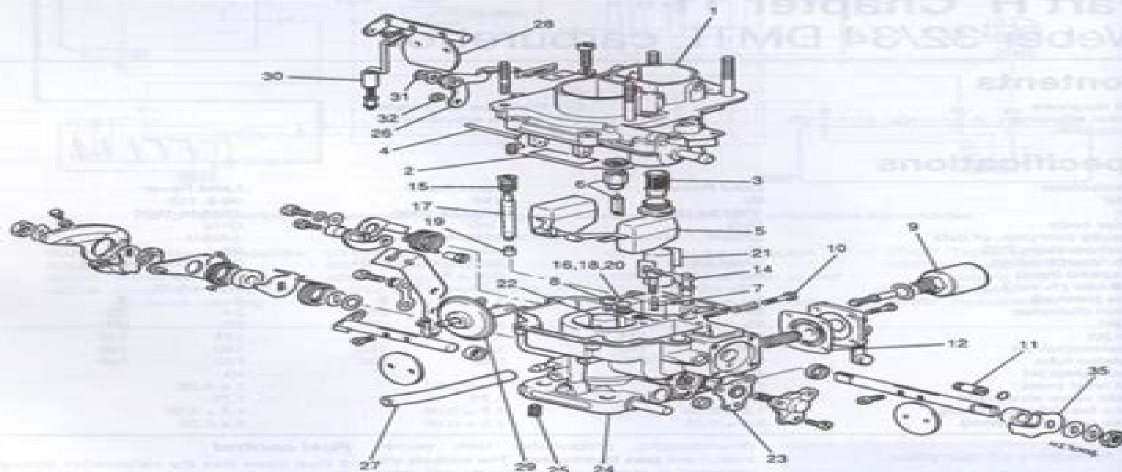
1.2 Weber DMTL carburettor
