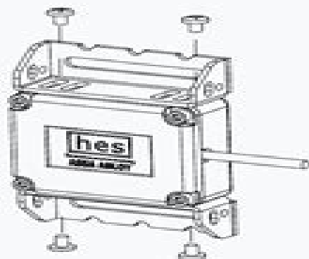
DIAGRAM 1: MOUNTING BRACKET INSTALLATION
